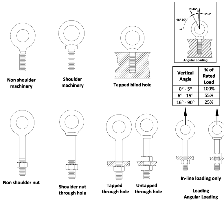
Figure 20 Eyebolts
