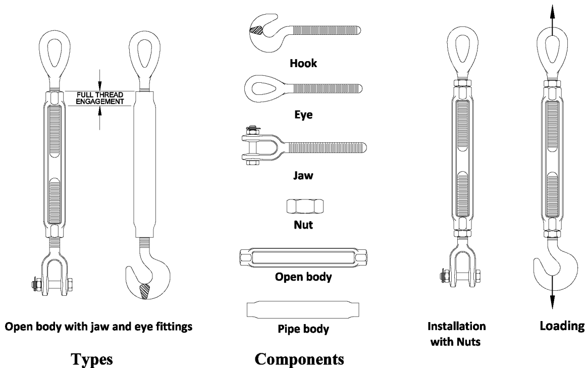
Figure 30 Turnbuckle Types
