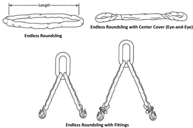
Figure 15 Synthetic Roundslings
