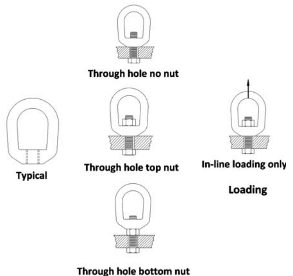
Figure 32 Eye Nuts
