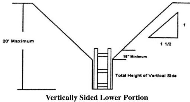
Figure N-12 Slope Configurations for Type C Soil Support or Shield System
