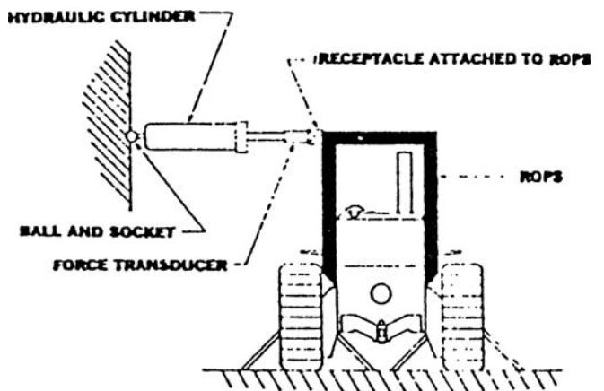
FIGURE V-4 Side-loading setup for crawler tractors and crawler loaders.
