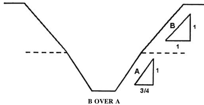
Figure N-13 EXCAVATIONS MADE IN LAYERED SOILS All excavations 20 feet or less in depth made in layered soils ((shall)) must have a maximum allowable slope for each layer as set forth below.
