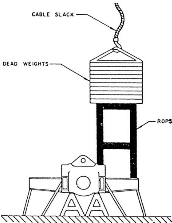
FIGURE V-1 Vertical loading setup for all types of equipment described in WAC 296-155-955(1).
