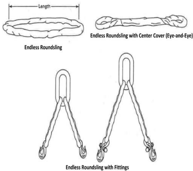
Figure 15 Synthetic Roundslings
