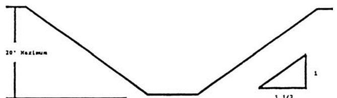
Simple Slope
