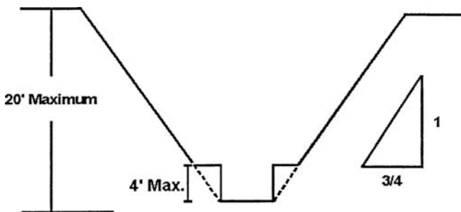
Simple Bench
