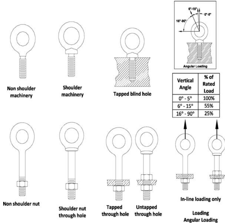
Figure 20 Eyebolts
