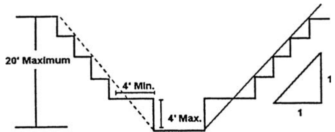
Multiple Bench
