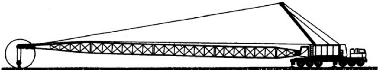
Figure 4. Pendant is in tension while connected to uppermost boom section, and no pins are to be removed.
