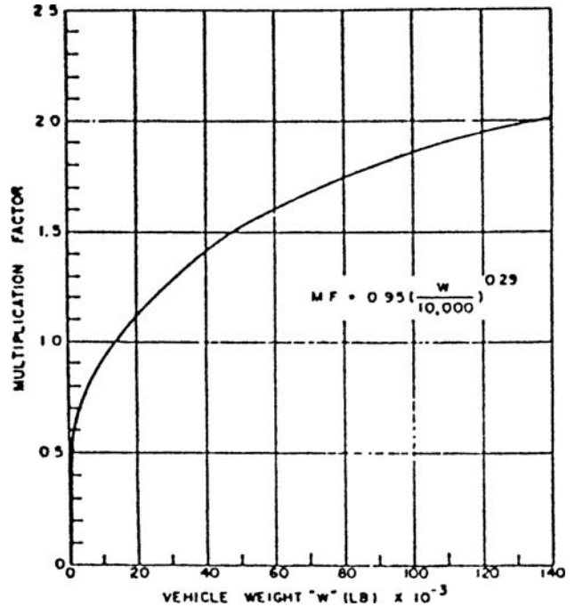
FIGURE V-10 Minimum horizontal load factor for self-propelled scrapers.
