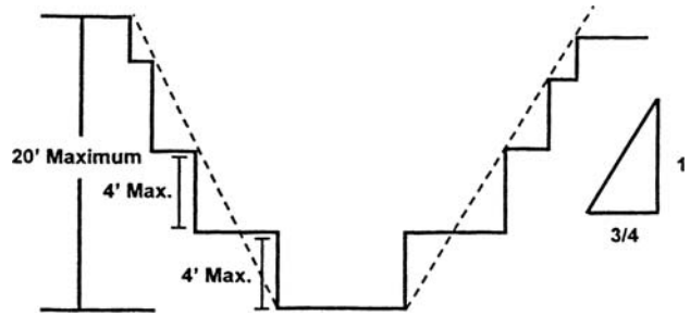
Multiple Bench
