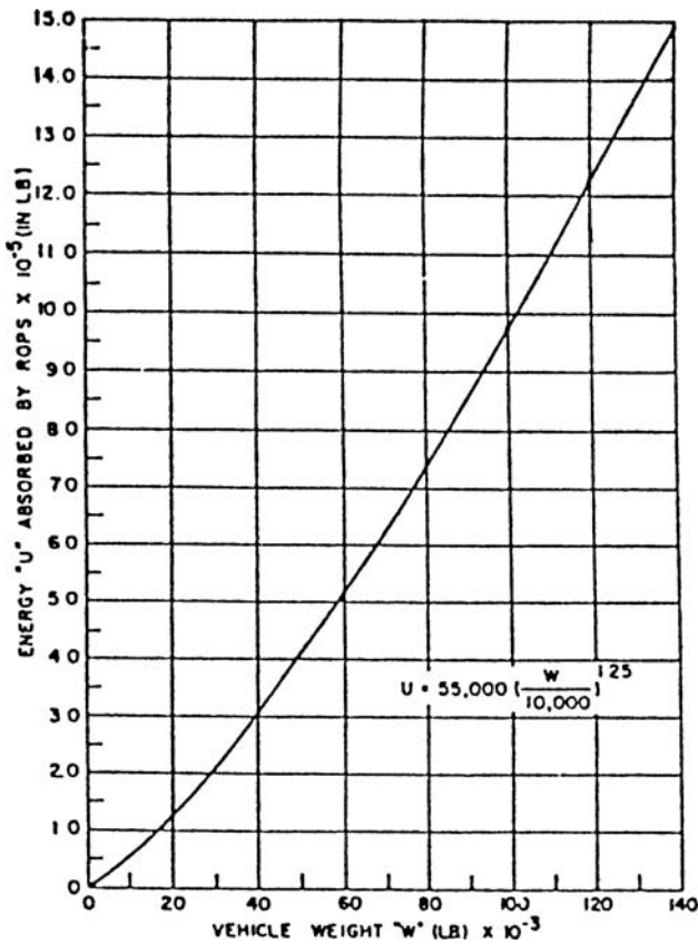
FIGURE V-9 Energy absorbed versus vehicle weight.
