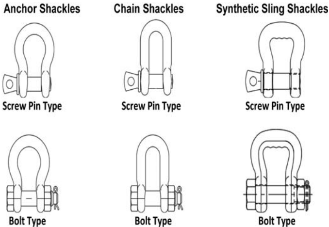
Figure 18 Shackle Types
