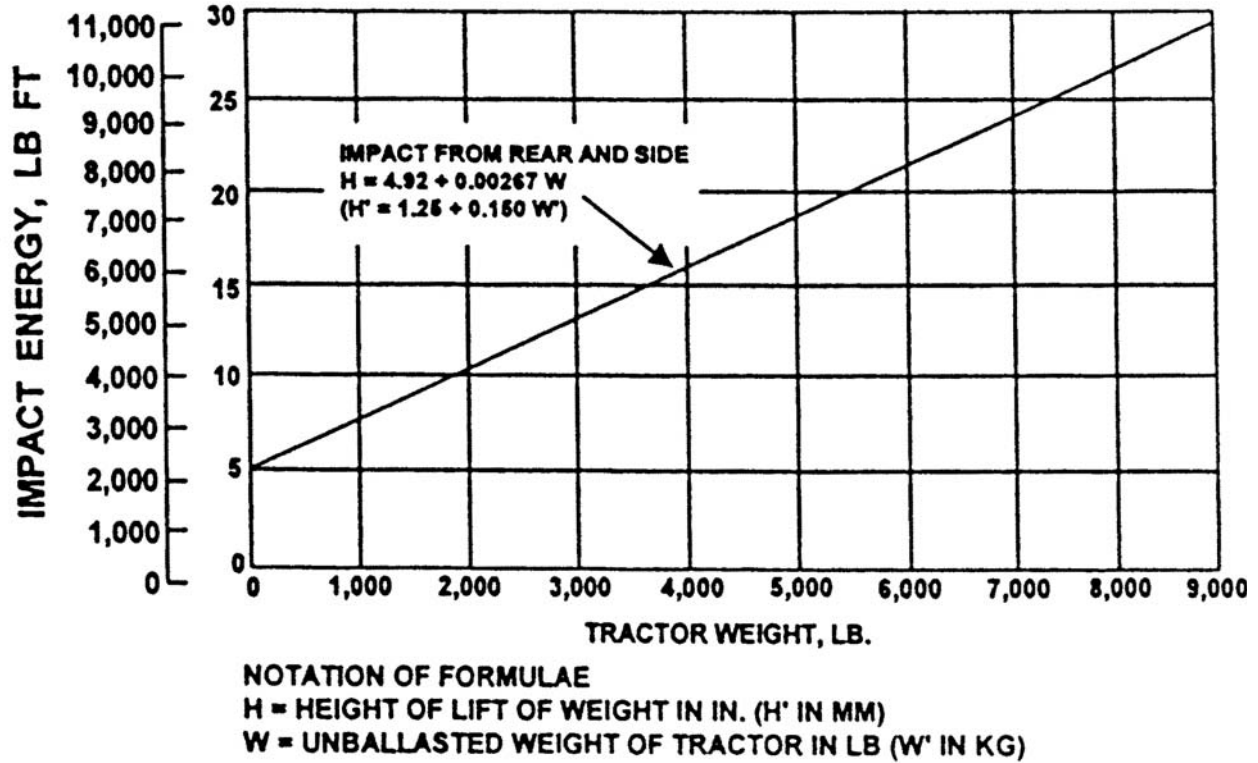
FIGURE V-14 Impact energy and corresponding lift height of 4,410 lb. (2,000 kg.) weight.
