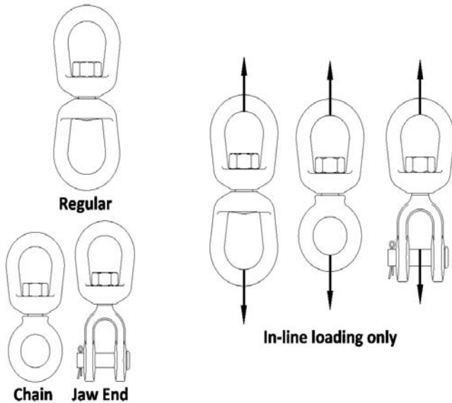
Figure 27 Swivels
