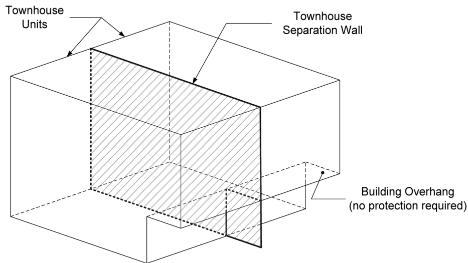
FIGURE R302.2(1) EXTENDED TOWNHOUSE SEPARATION WALL
