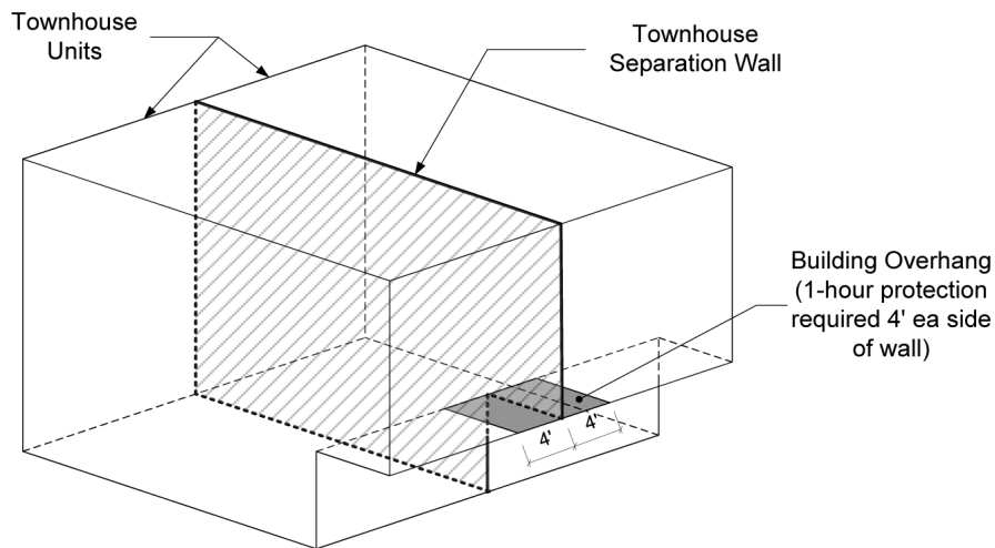
FIGURE R302.2(2) TOWNHOUSE SEPARATION OVERHANG PROTECTION
