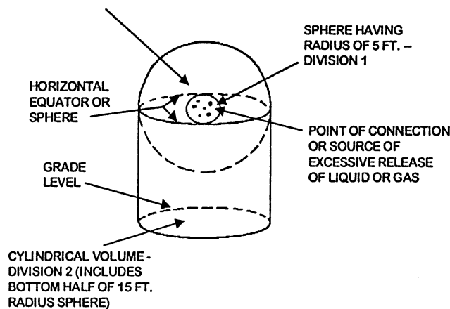
SPHERE HAVING RADIUS OF 15 FT. -- DIVISION 2
