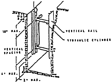
Figure N-24, Pneumatic/hydraulic Shoring
