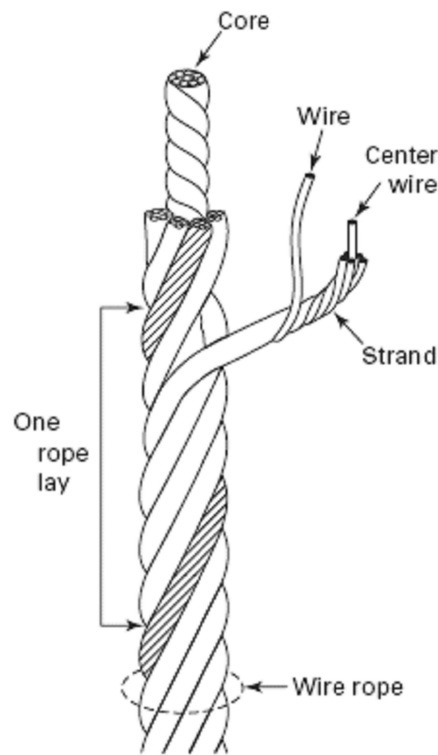
Figure 1 - Wire Rope
