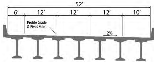
Exhibit 6: Typical Section Concept – Four-lane Option
