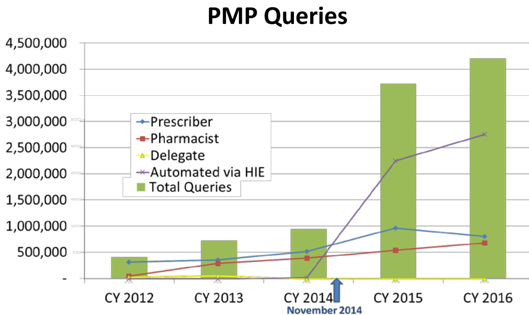
Figure 2: PMP Queries
